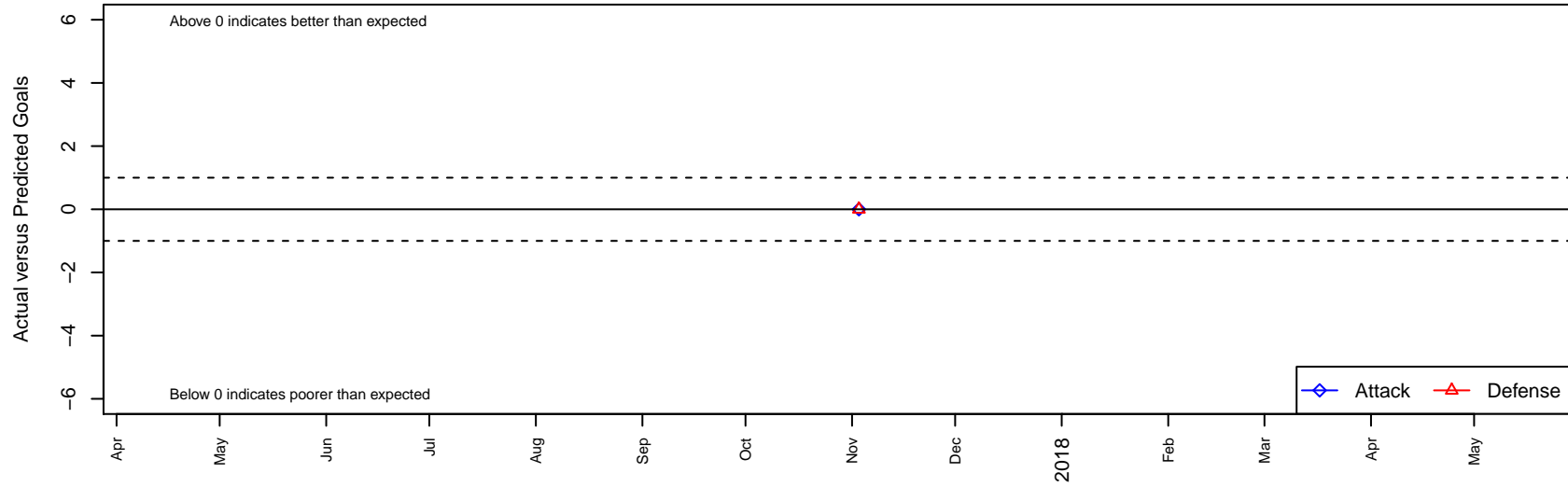
FC Boulder USSDA B05 Dots are actual minus expected GF (blue circles) and GA (red triangles). Blue line is smoothed change in attack strength. Red is smoothed change in defense strength.
